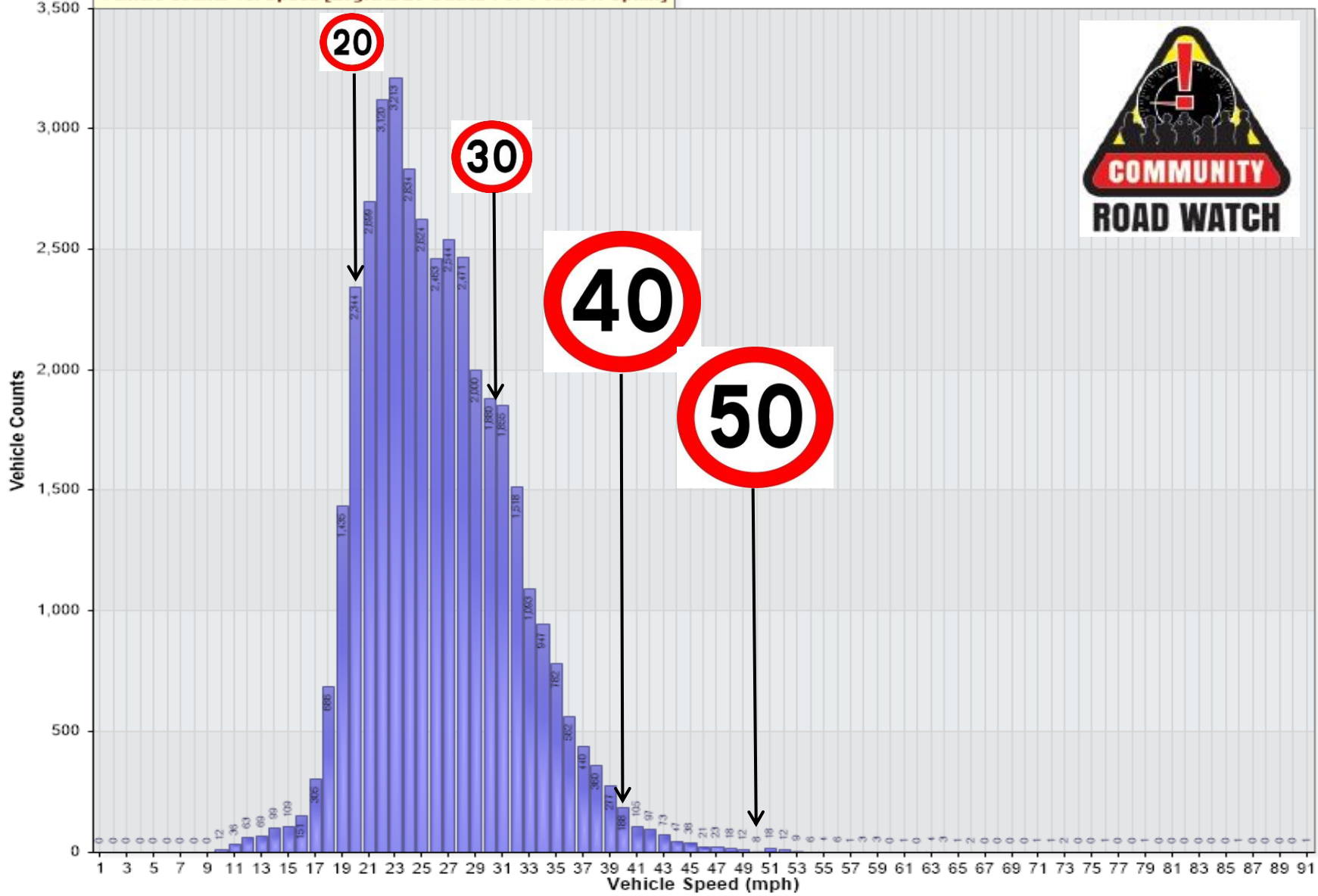
Vehicle Counts Vs. Speed [LogHAD20-StnRd-FUPT-Jan24: Uphill]
