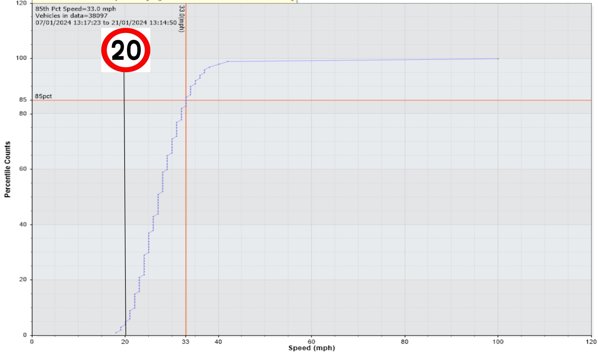
Percentile Counts Vs. Speed for [LogHAD20-StnRd-FUPT-Jan24: Downhill]
