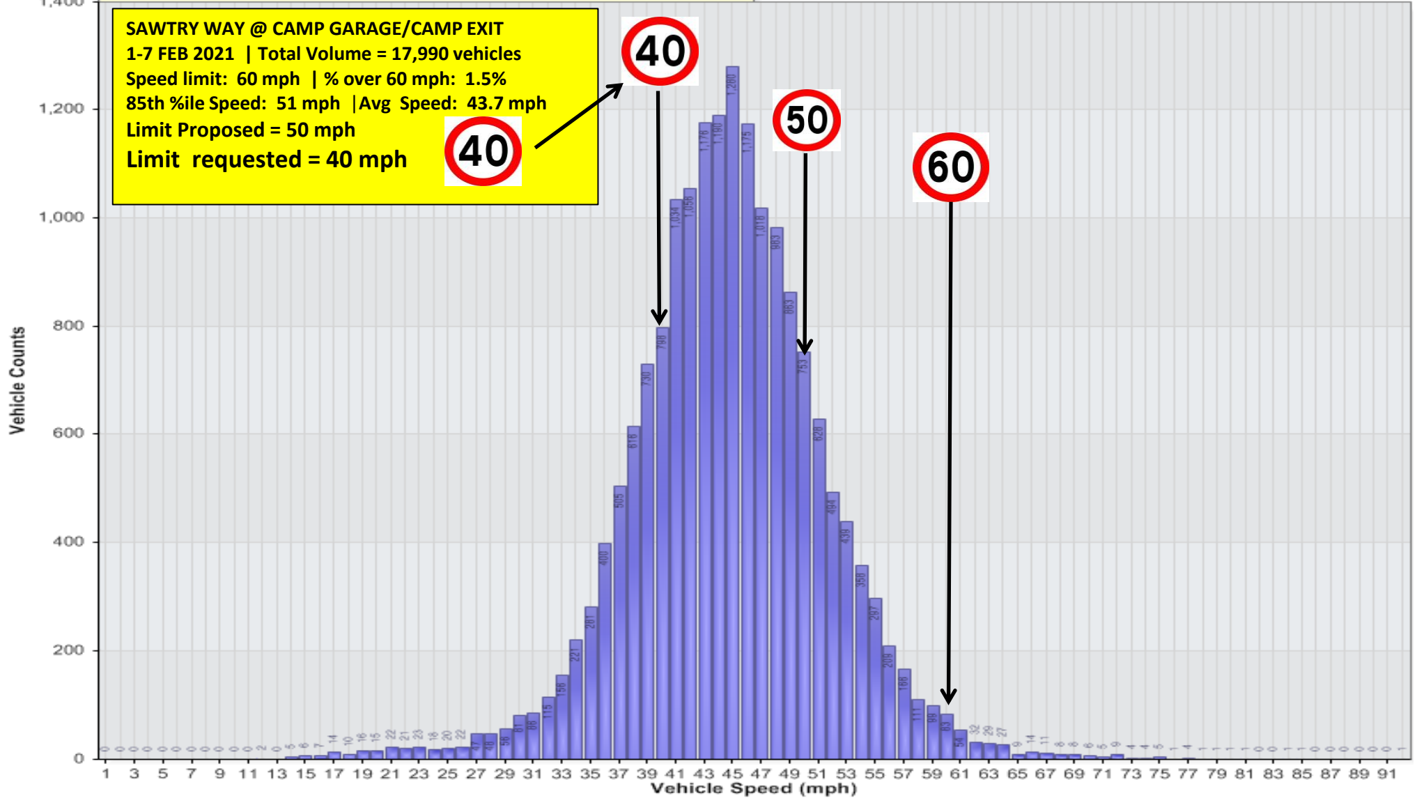
Vehicle Counts Vs. Speed [LogLHI-CampGarageFeb21: West-Bound]
