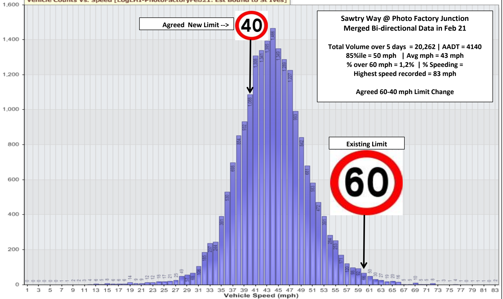
Vehicle Counts Vs. Speed [LogLHI-PhotoFactoryFeb21: Est Bound to St Ives]
