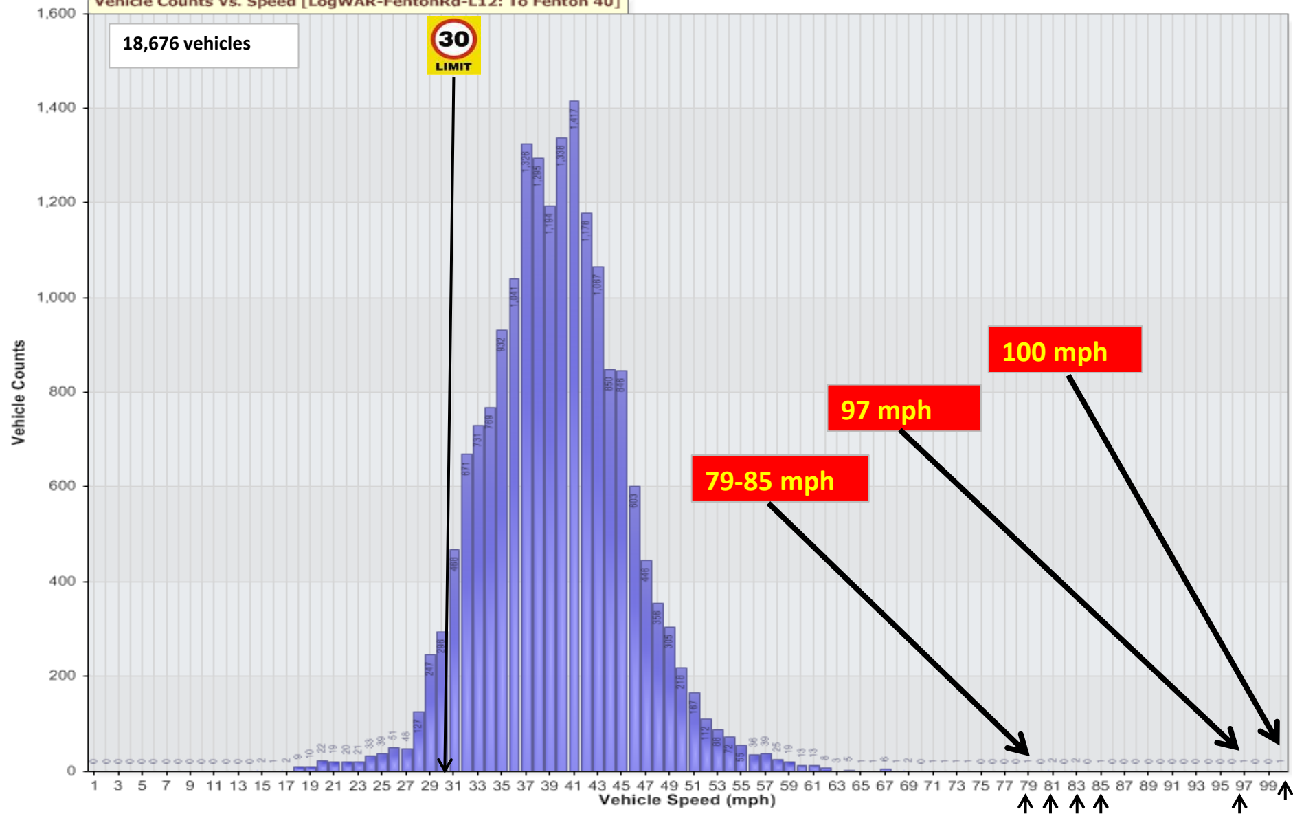
Vehicle Counts Vs. Speed [LogWAR-FentonRd-L12: To Fenton 40]
