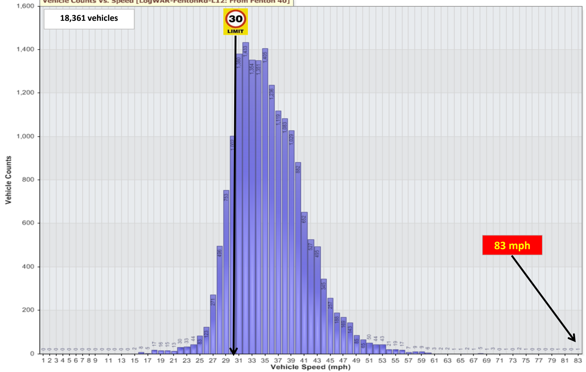
Vehicle Counts Vs. Speed [LogWAR-FentonRd-L12: From Fenton 40]
