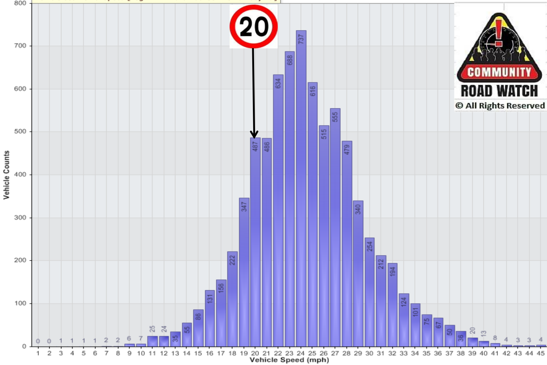
Vehicle Counts Vs. Speed [LogWAR-HDaleAtSchool: To Ramsey Rd]
