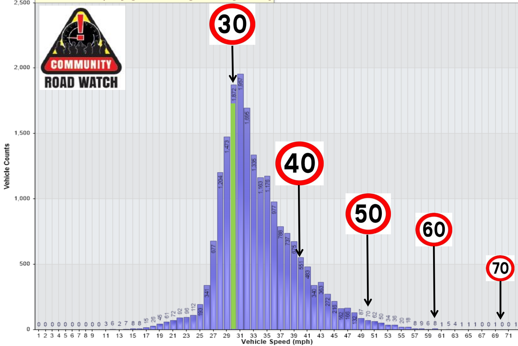
Vehicle Counts Vs. Speed [LogWAR-RR-FIB-Aug23: Incoming Direction]
