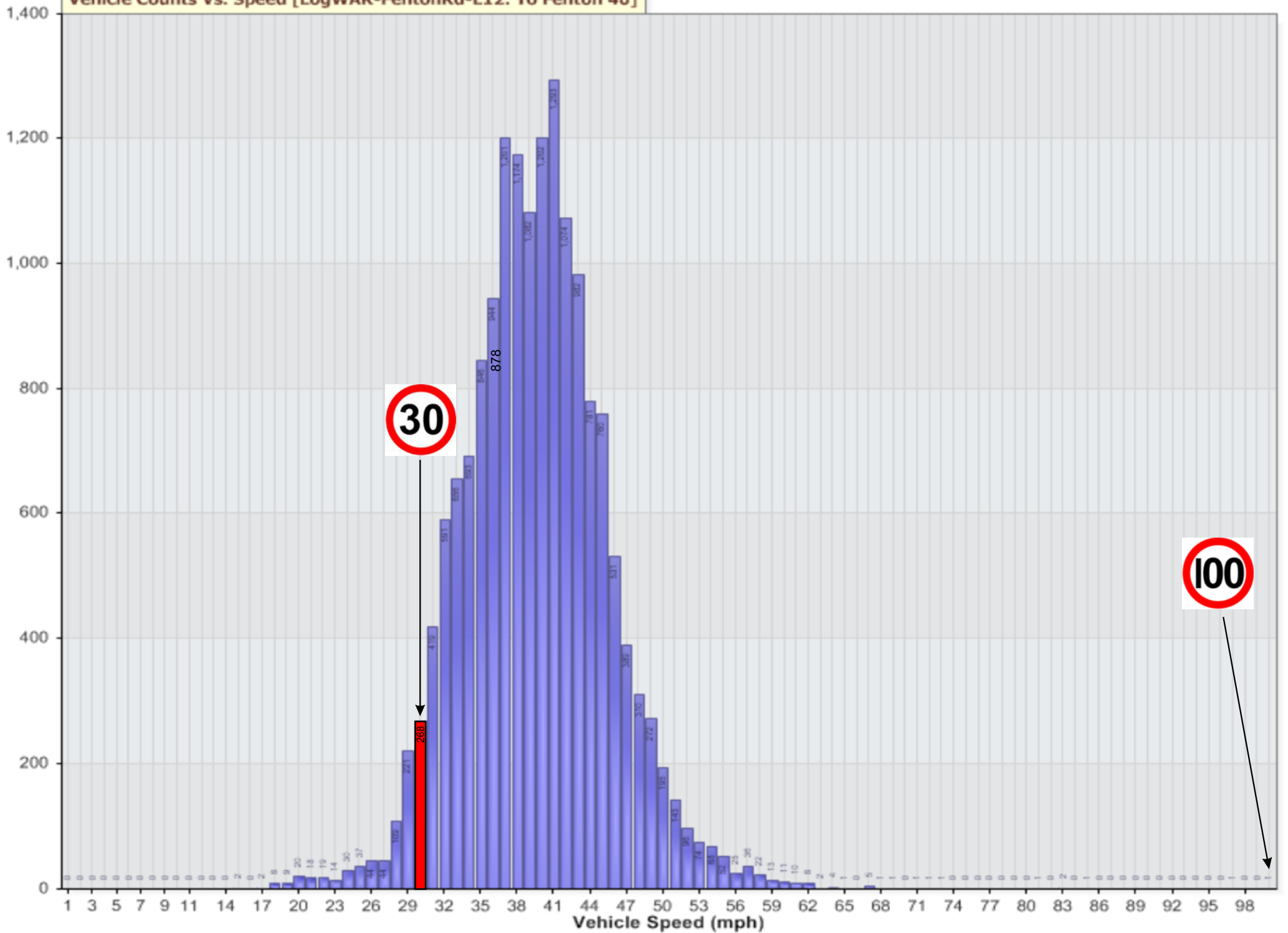
Vehicle Counts Vs. Speed [LogWAR-FentonRd-L12: To Fenton 40]
